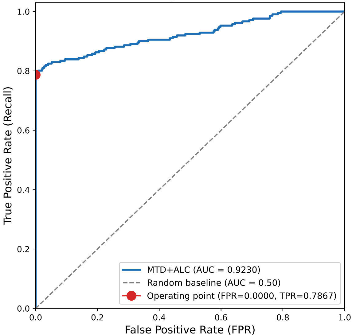
ROC Curve — BigVul (held-out test set)
