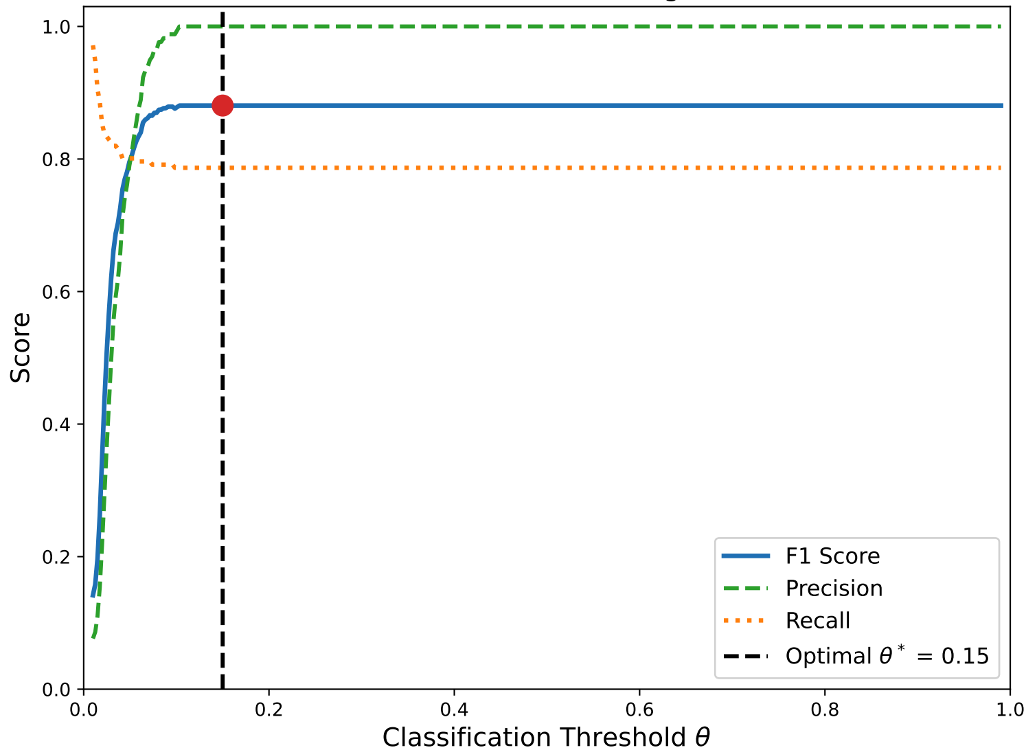
Precision, Recall & F1 vs Threshold — BigVul (held-out test set)
