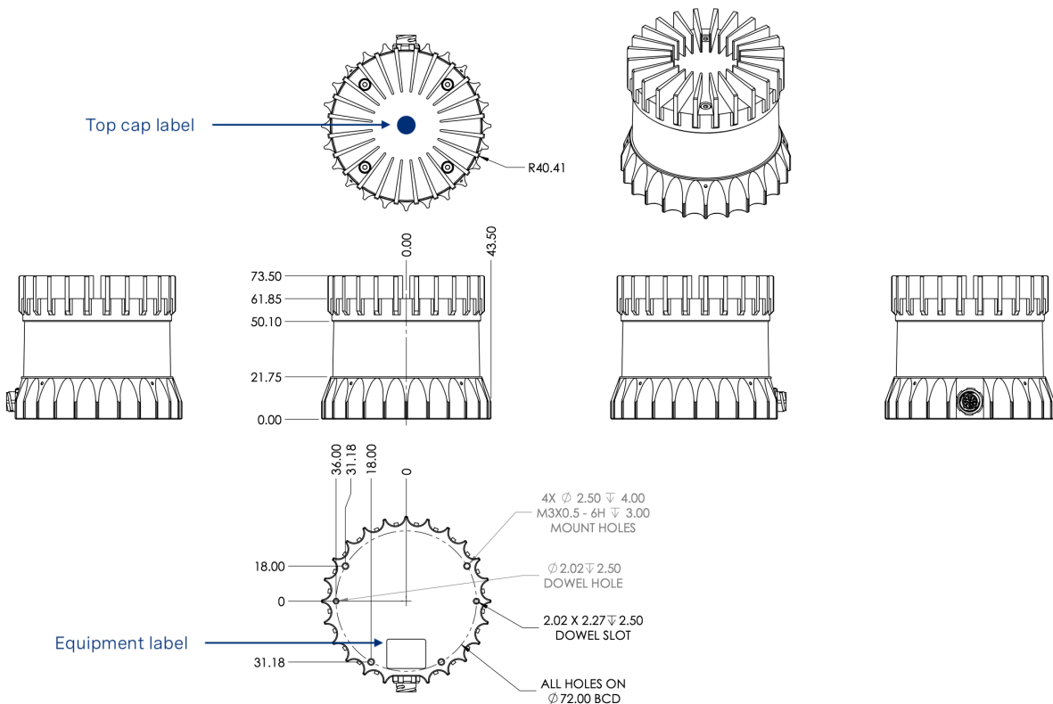
Figure 4.1: Sensor Components
