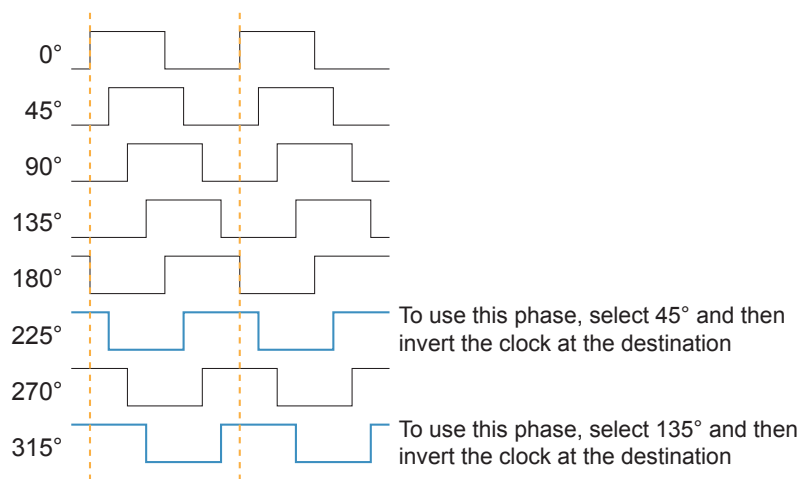
Figure 39: PLL Clock Phases
