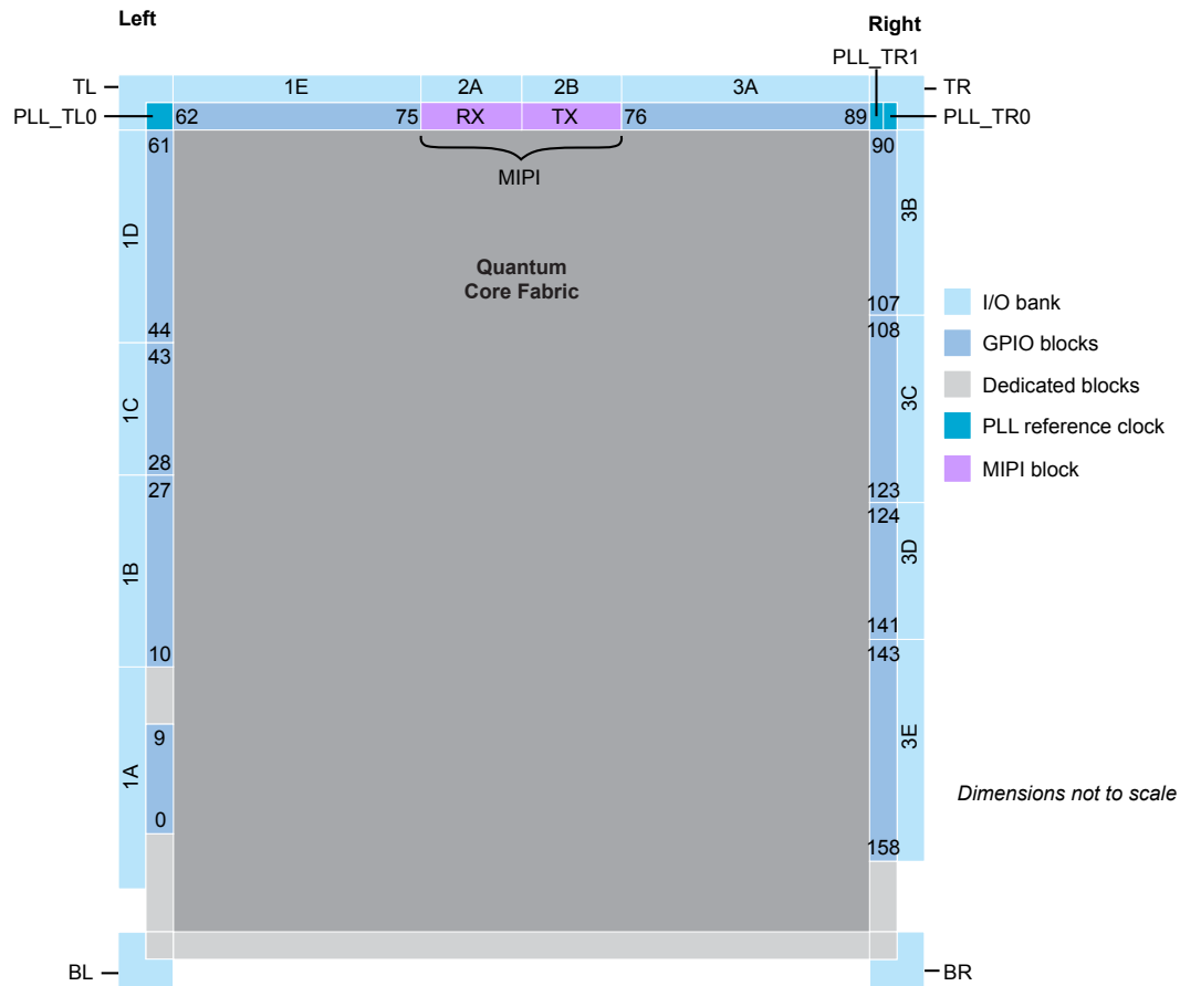
Figure 42: T20 FPGAs
