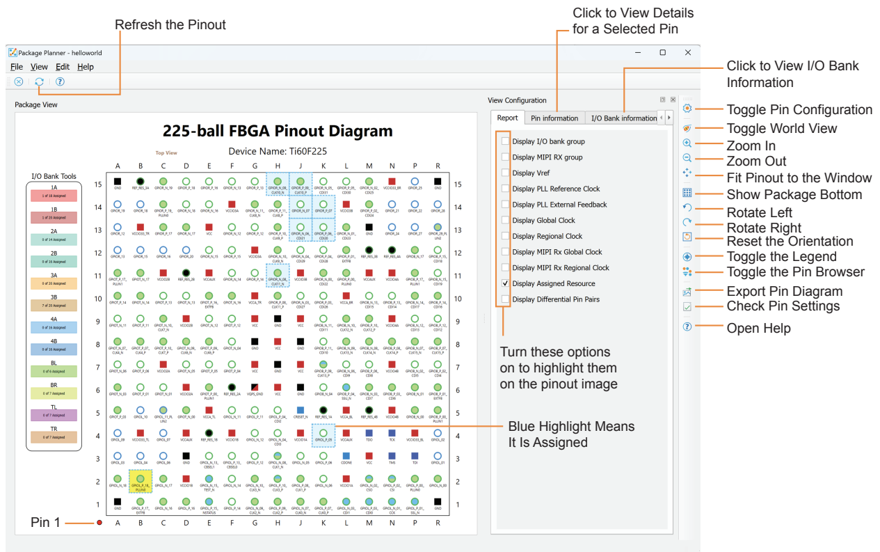
Figure 6: Package Planner
