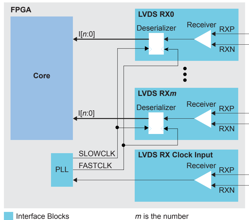
Figure 26: Complete LVDS RX Interface Block Diagram
