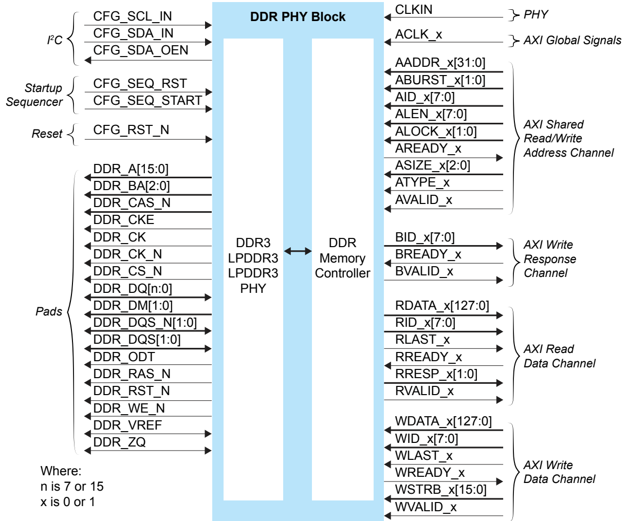
Figure 12: (T20, T35) DDR DRAM Block Diagram
