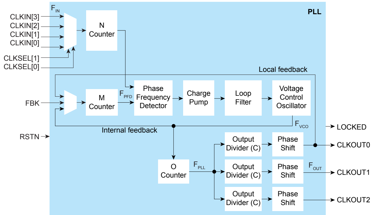
Figure 37: Advanced PLL Block Diagram
