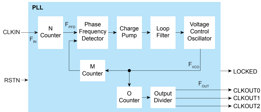
Figure 35: Trion PLL Block Diagram
