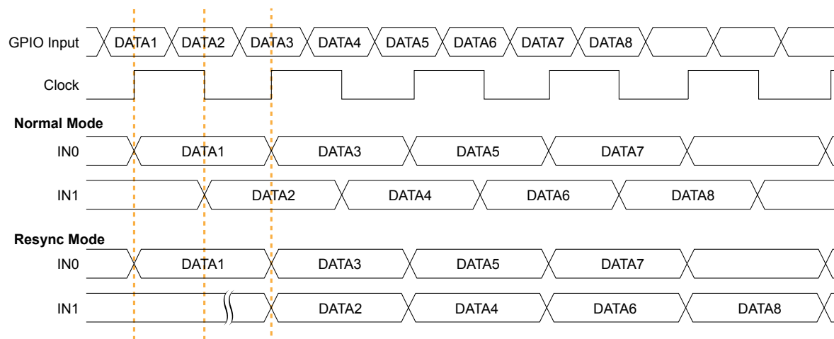
Figure 17: DDIO Input Timing Waveform
