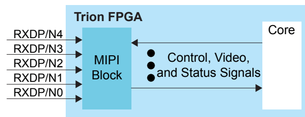
Figure 31: MIPI RX Interface Block Diagram
