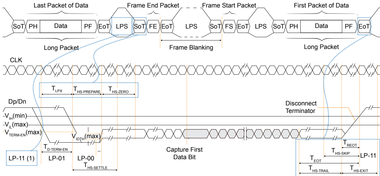
Figure 32: High-Speed Data Transmission in Bursts Waveform
