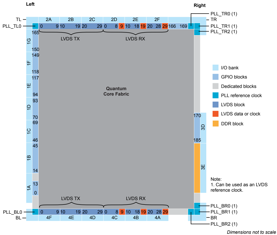
Figure 50: T55, T85, and T120 FPGAs
