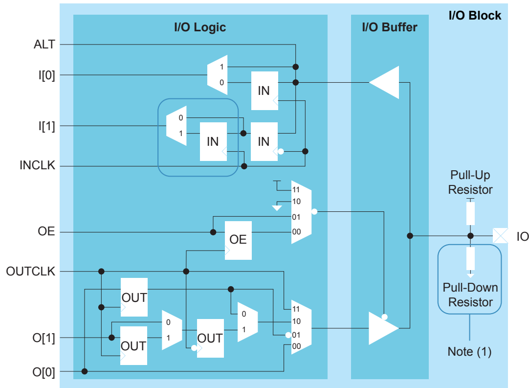
Figure 16: I/O Interface Block
