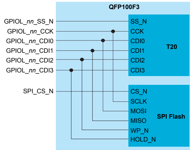
Figure 40: Connections between FPGA and SPI Flash Device inside the Package
