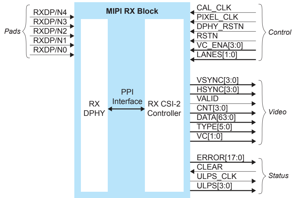
Figure 30: MIPI RX x4 Block Diagram
