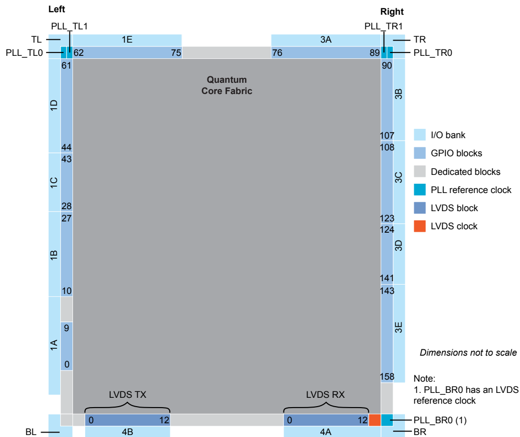
Figure 46: T35 FPGAs
