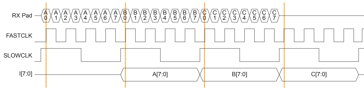
Figure 24: LVDS RX Timing Example Serialization Width of 8
