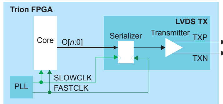
Figure 19: LVDS TX Interface Block Diagram
