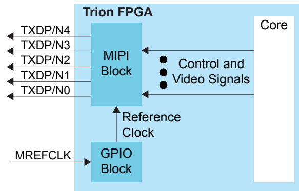
Figure 29: MIPI TX Interface Block Diagram
