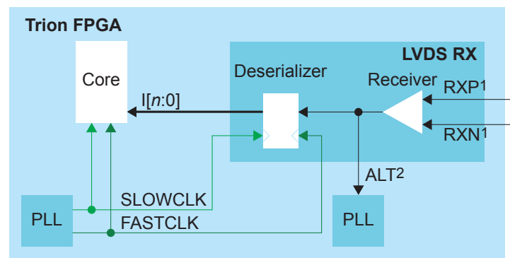
Figure 23: LVDS RX Interface Block Diagram
