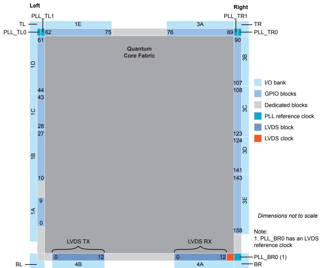
Figure 43: T8, T13, and T20 FPGAs
