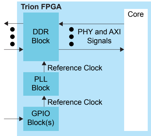
Figure 14: DDR DRAM Interface Block Diagram
