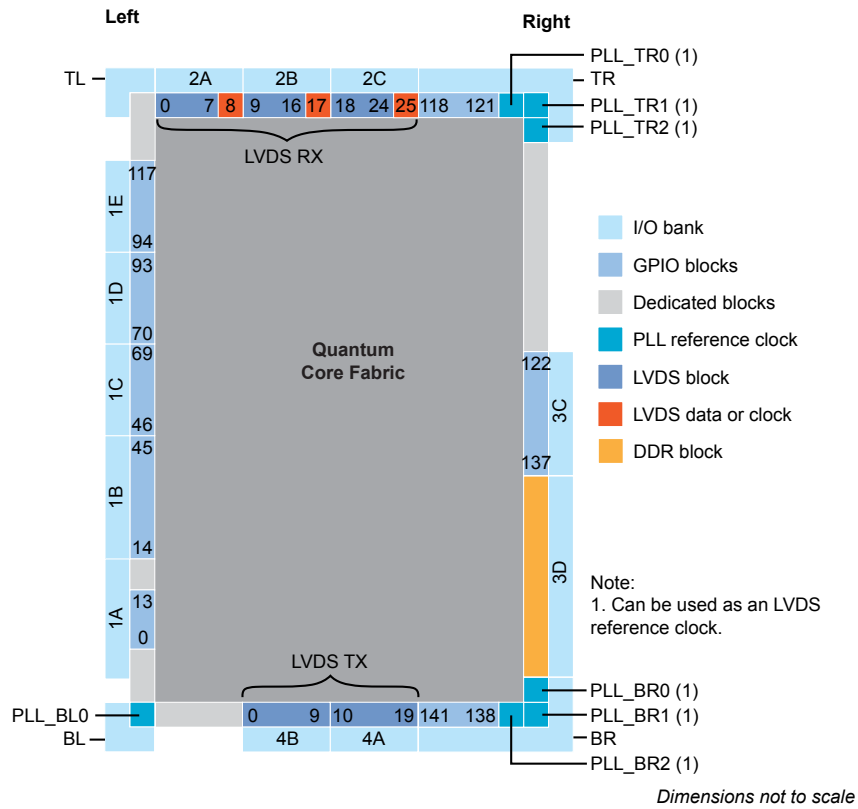
Figure 49: T20 and T35 FPGAs
