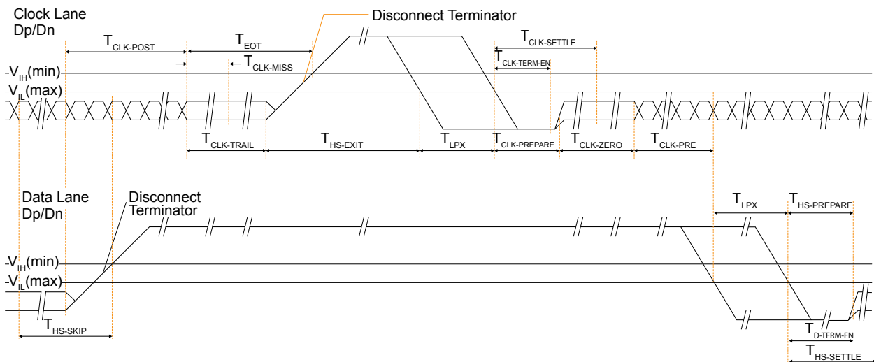
Figure 33: Switching the Clock Lane between Clock Transmission and Low Power Mode Waveform
