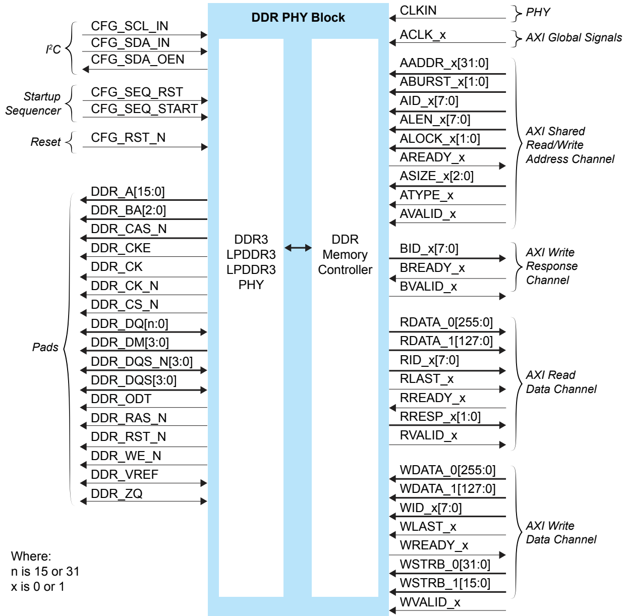
Figure 13: (T55, T85, T120) DDR DRAM Block Diagram
