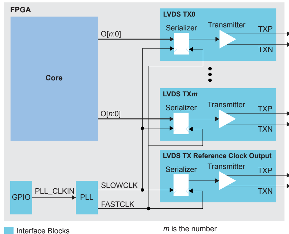
Figure 25: Complete LVDS TX Interface Block Diagram
