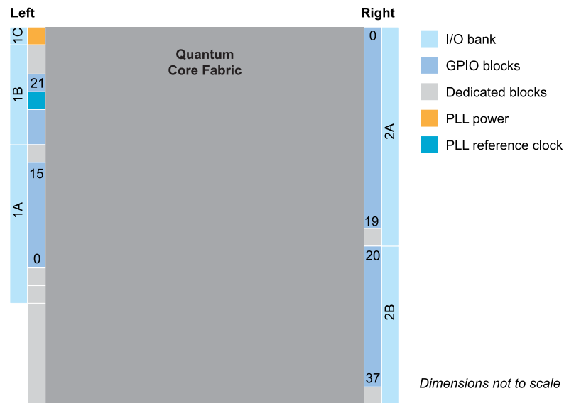
Figure 41: T4 and T8 FPGAs
