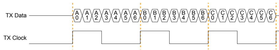
Figure 22: LVDS Timing Data and Clock Relationship Width of 7 (Parallel Clock Division=1)
