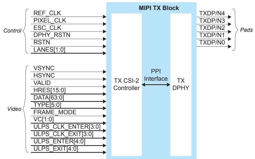
Figure 28: MIPI TX x4 Block Diagram
