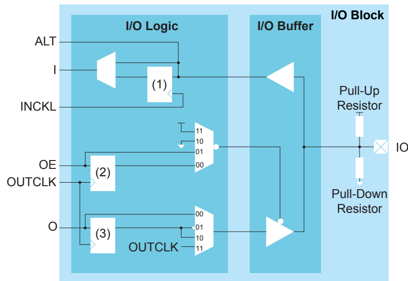
Figure 15: T8/T4 I/O Interface Block
