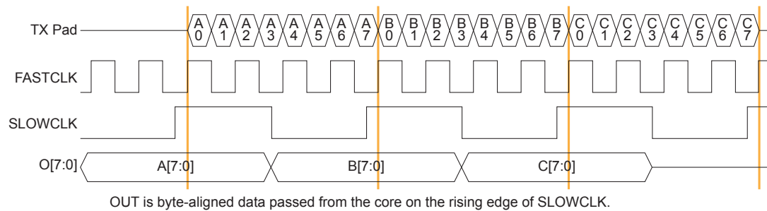
Figure 21: LVDS Timing Data and Clock Relationship Width of 8 (Parallel Clock Division=1)
