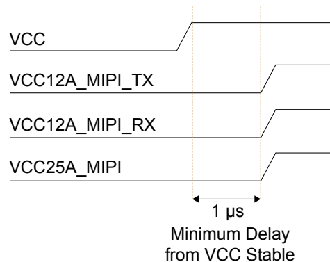
Figure 34: MIPI Power Up Sequence
