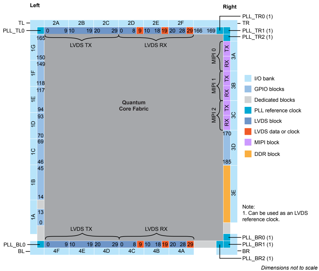
Figure 51: T55, T85, and T120
