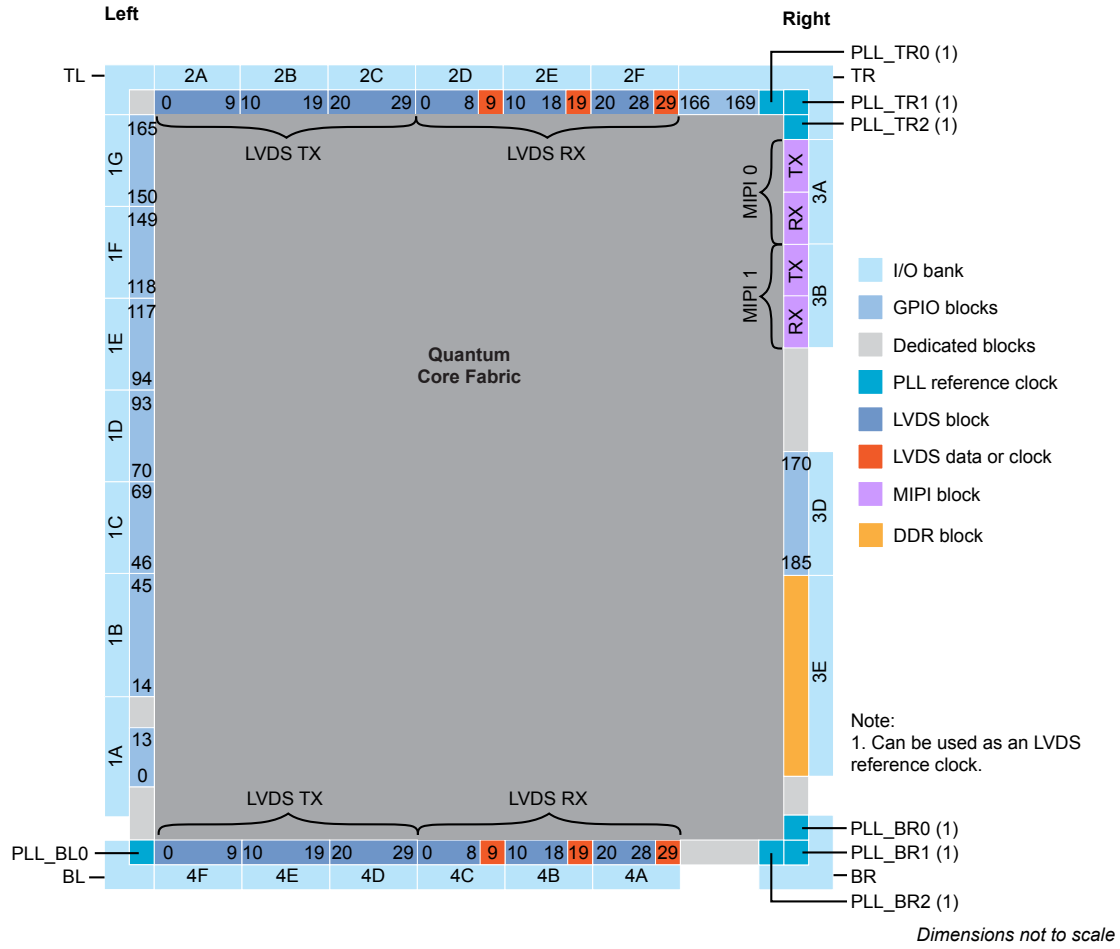
Figure 48: T55, T85, T120
