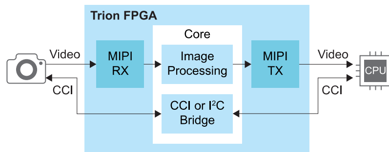
Figure 27: MIPI Example System
