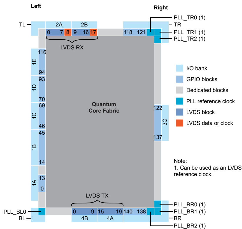
Figure 46: T35 FPGAs
