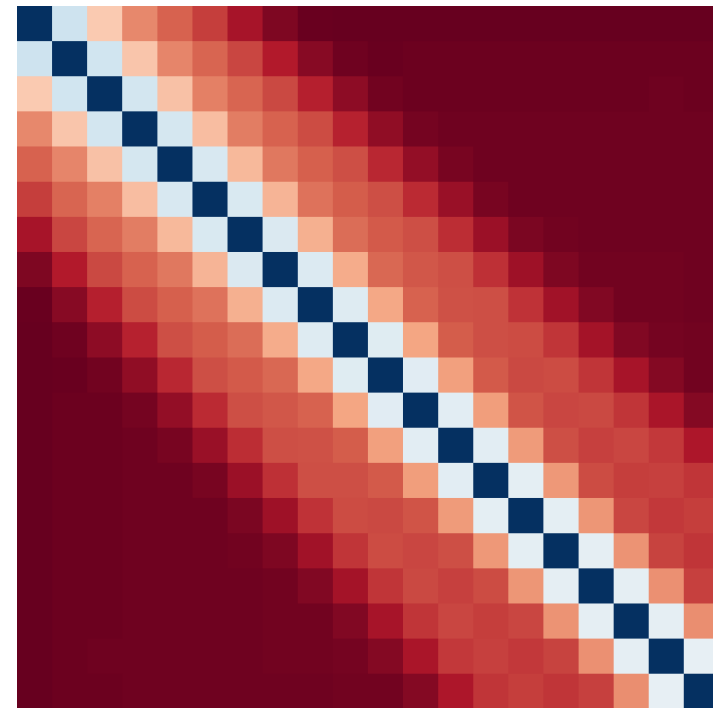
L2 distances
