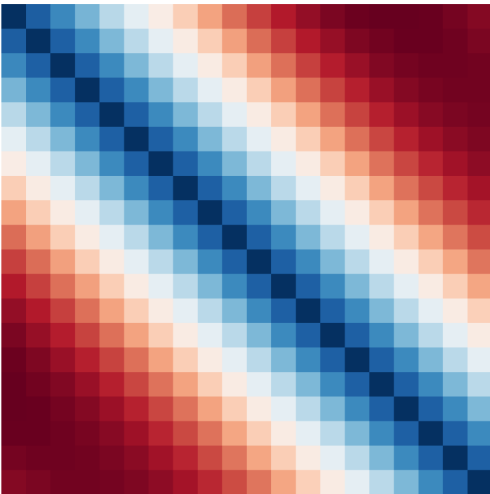
W1 distances
