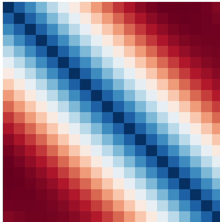
W2 distances
