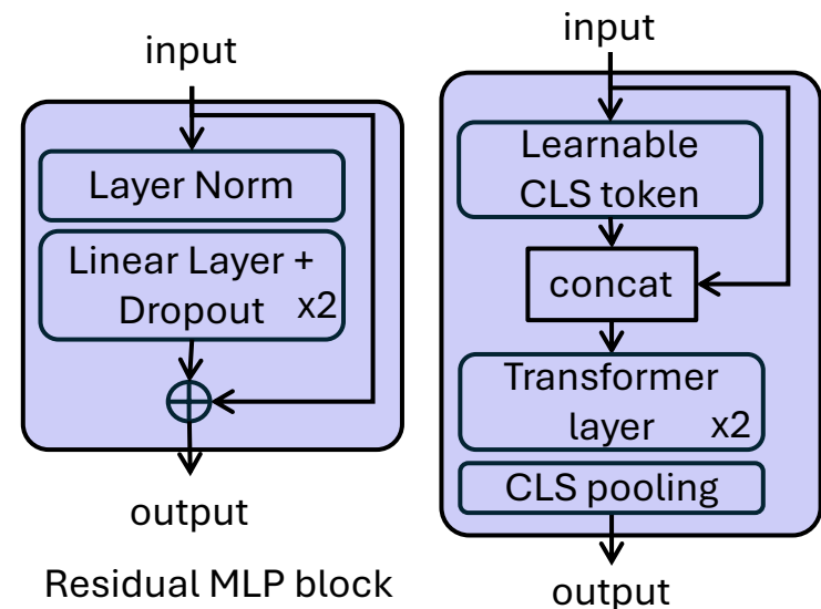
Set Attention Encoder
