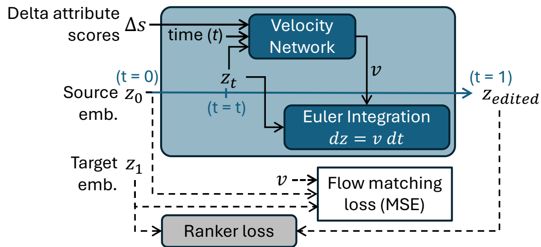
(b) RAFT model training.
