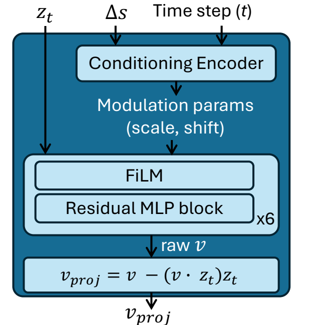
(c) Velocity Network Architecture
