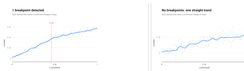
Figure 6: The same subtle knee at two noise levels: low noise (left) is detected with one breakpoint, high noise (right) abstains with zero, the same true shape underneath both panels.
