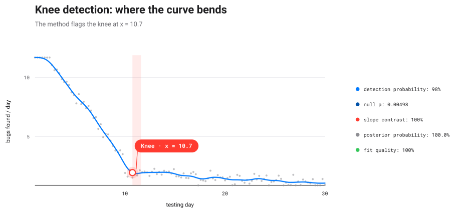
Figure 11: Bugs found per day of testing, with elbow_helper.robust_knee 's detected knee (dashed red line and callout) at day 10.7, one day past the true break at day 10.
