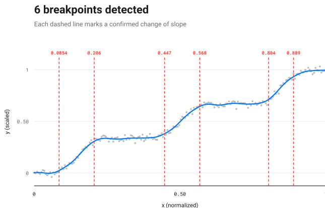
Figure 5: A smooth staircase built from three logistic sigmoids, with elbow_helper.robust_knees 's six detected breakpoints (dashed red lines) each bracketing one rise's start and end.
