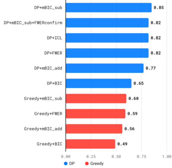
Figure 2: Left: exact- k accuracy, ranked, for every dynamic-program (blue) and greedy (red) combination with the four several-knee criteria this note derives, BIC, mBIC, ICL, and the FWER sequential test, measured on the same synthetic benchmark. Every DP-based method outranks its greedy counterpart. Right: the same ten methods' false-positive rate on genuinely flat data, plain BIC the clear outlier on both sides regardless of search strategy.
