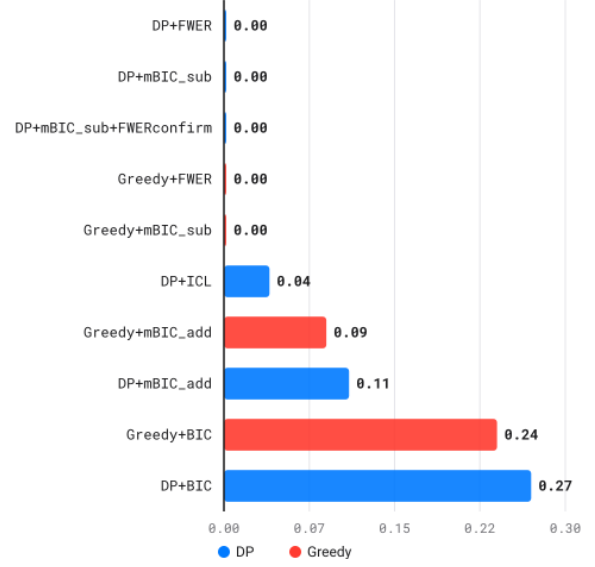
Figure 2: Left: exact- k accuracy, ranked, for every dynamic-program (blue) and greedy (red) combination with the four several-knee criteria this note derives, BIC, mBIC, ICL, and the FWER sequential test, measured on the same synthetic benchmark. Every DP-based method outranks its greedy counterpart. Right: the same ten methods' false-positive rate on genuinely flat data, plain BIC the clear outlier on both sides regardless of search strategy.
