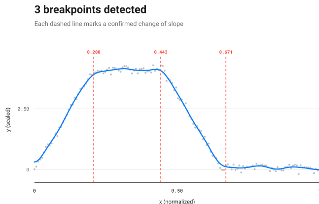
Figure 4: A mountain curve with elbow_helper.robust_knees ’s three detected breakpoints (dashed red lines): up, flat, down, flat, recovered without any curve/direction argument.
