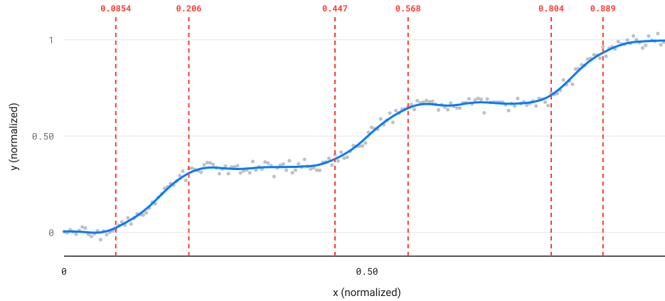
Figure 3: A smooth staircase built from three logistic sigmoids, with elbow_helper.robust_knees 's six detected breakpoints (dashed red lines) each bracketing one rise's start and end.
