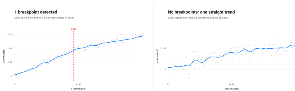
Figure 4: The same subtle knee at two noise levels: low noise (left) is detected with one breakpoint, high noise (right) abstains with zero, the same true shape underneath both panels.
