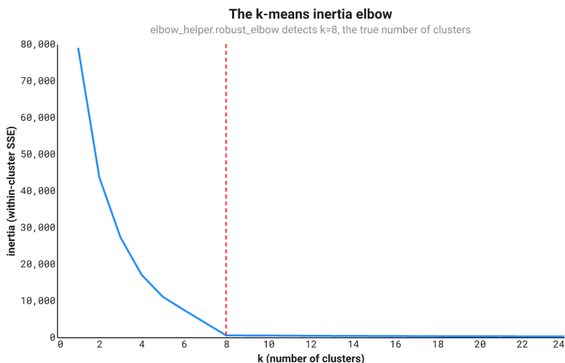
The k-means inertia curve, with elbow_helper.robust_elbow 's detected elbow (dashed red line) at k=8 , the true number of clusters.
