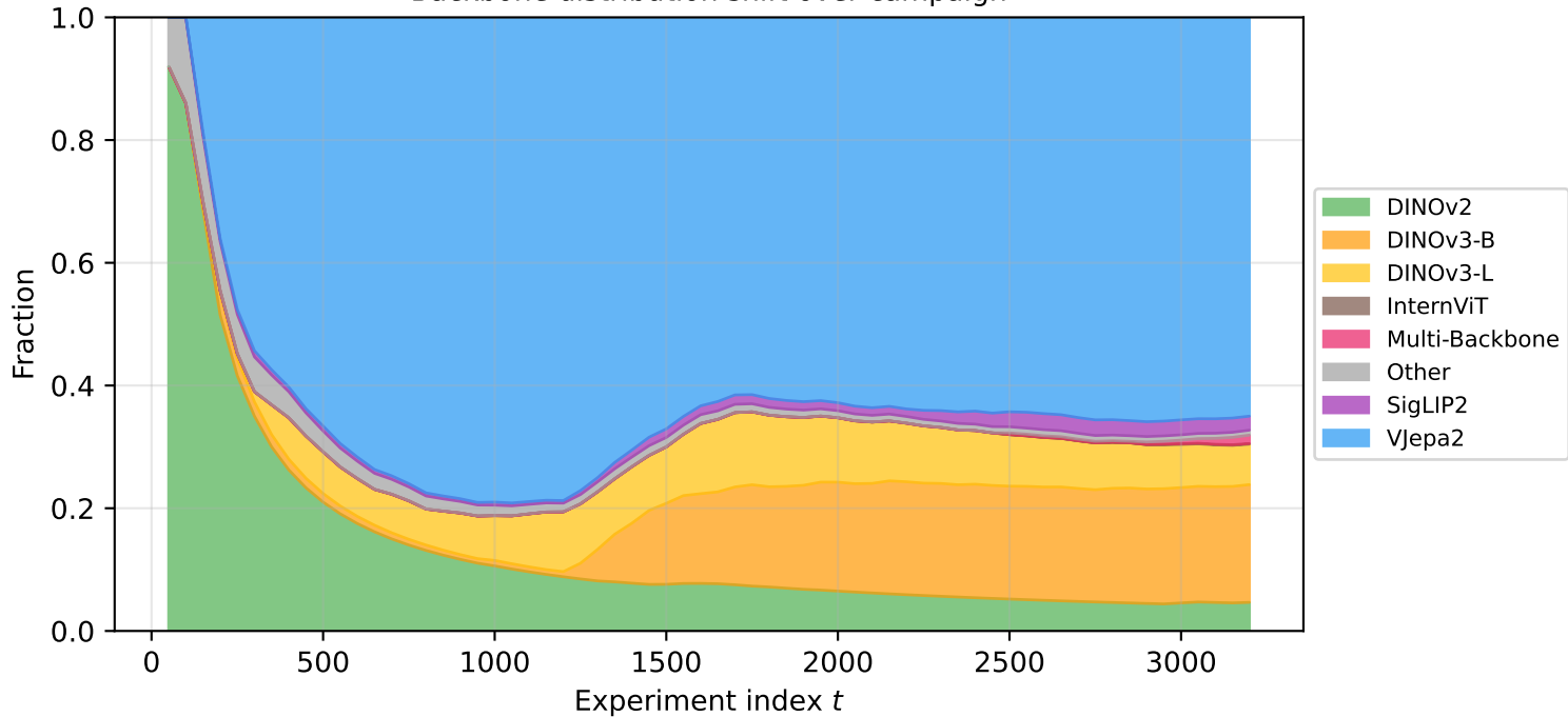
Backbone distribution shift over campaign
