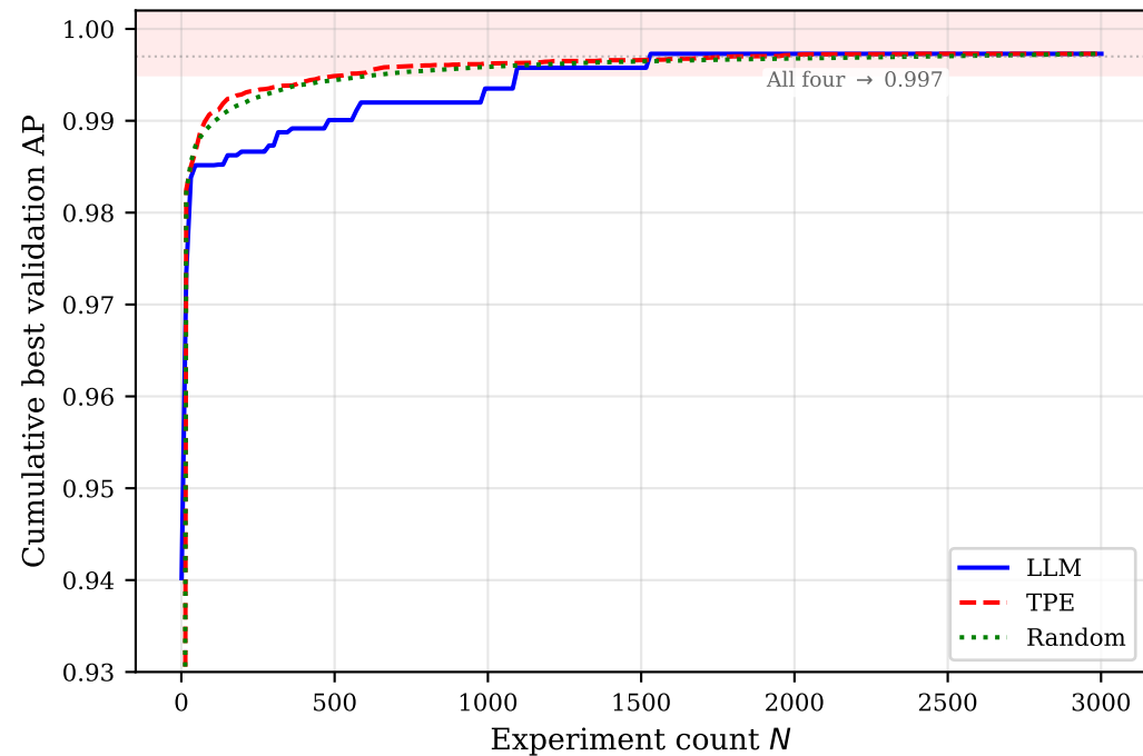
(a) Validation AP (saturated proxy)
