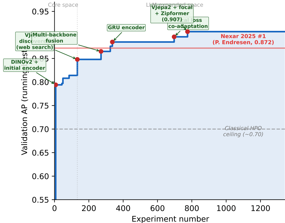
(a) Dashcam collision: SSC hill-climbing
