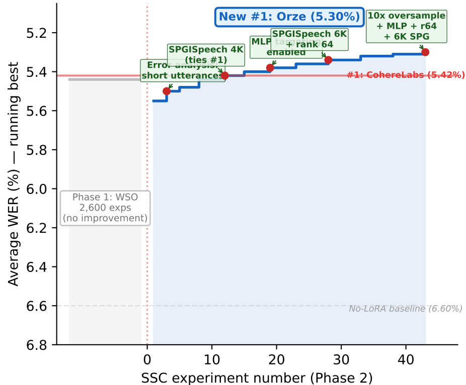
(b) ASR: SSC hill-descending
