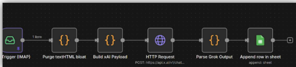
TheDeadlyConsulting.com Job Board Agentic Node Workflow
