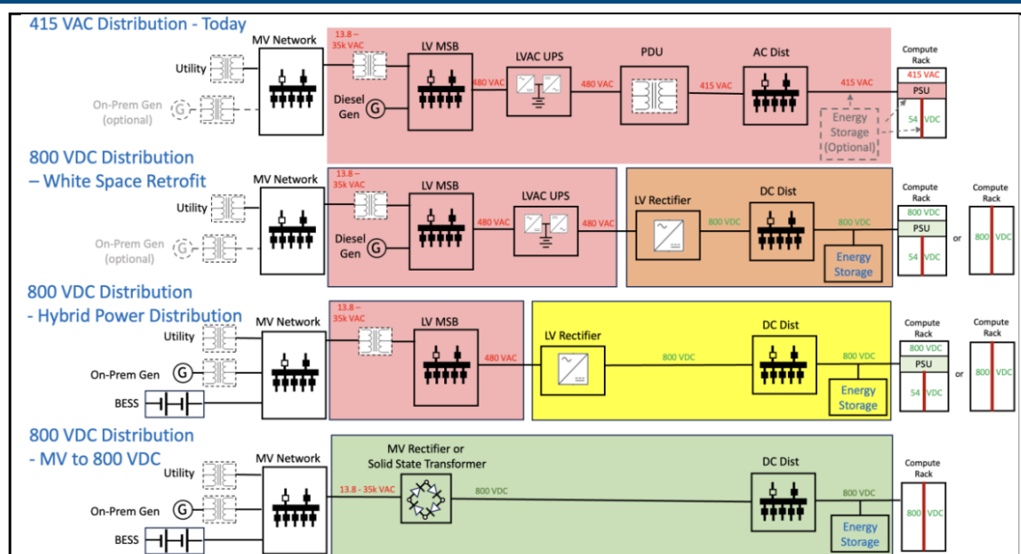
Figure 10: Datacenter architecture over time
