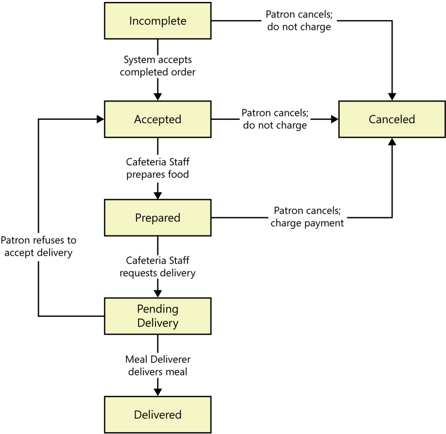
FIGURE C-4 State-transition diagram for meal order status.
