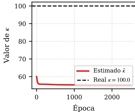
(c) Taxa Cinética \hat{\kappa}
