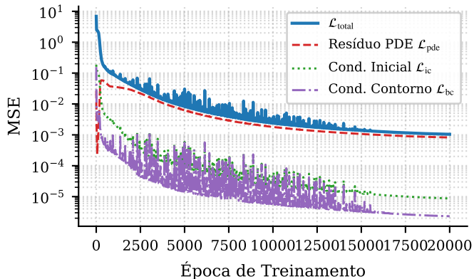
(a) Burgers 2D ( \nu = 0.01 )
