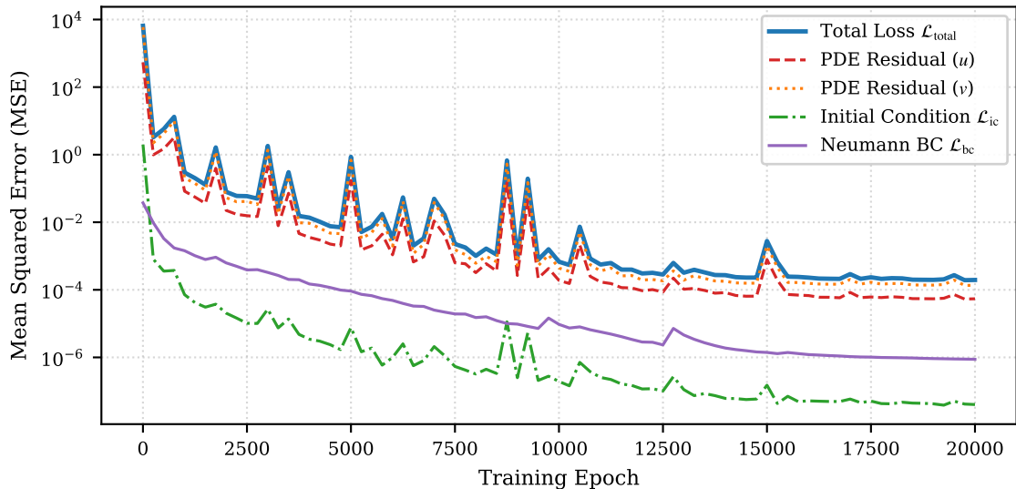
PINN Loss Convergence Analysis (20000 Epochs on NVIDIA GeForce RTX 3050 Laptop GPU)
