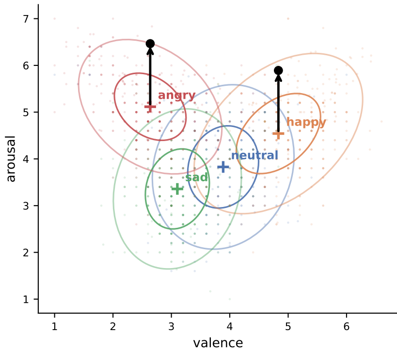
raw space: v - \mu_c
