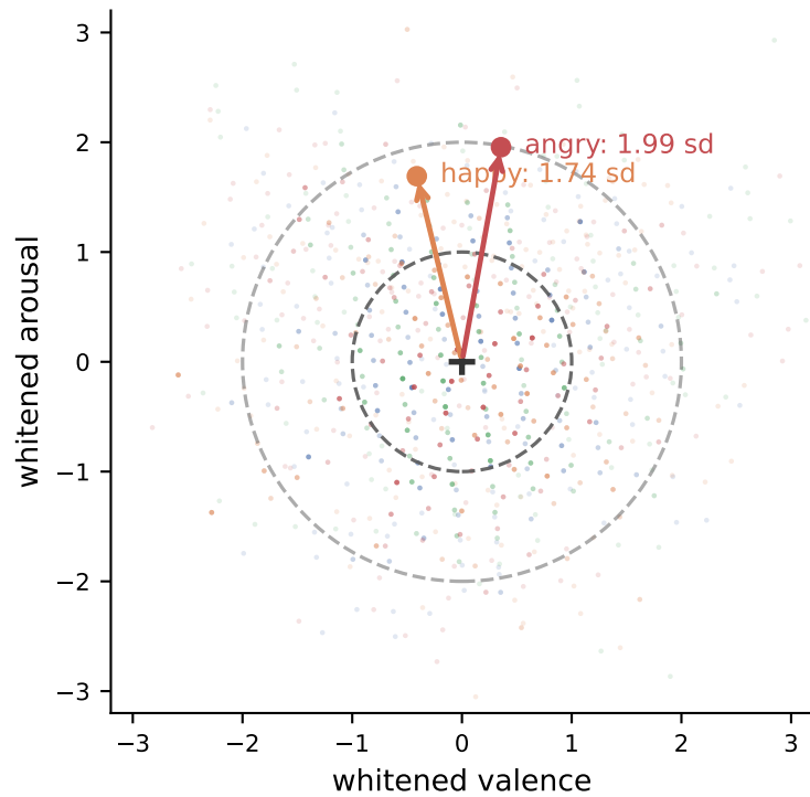
whitened: W_c(v - \mu_c)
