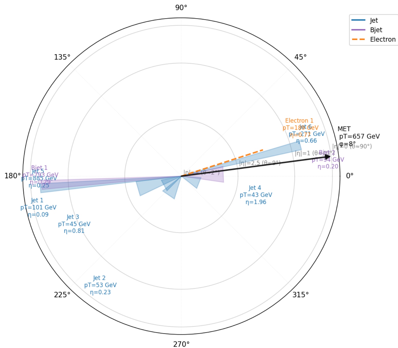
ATLAS Open Data: Z'(2\text{ TeV}) \rightarrow t\bar{t} (boosted) Event# 2736
