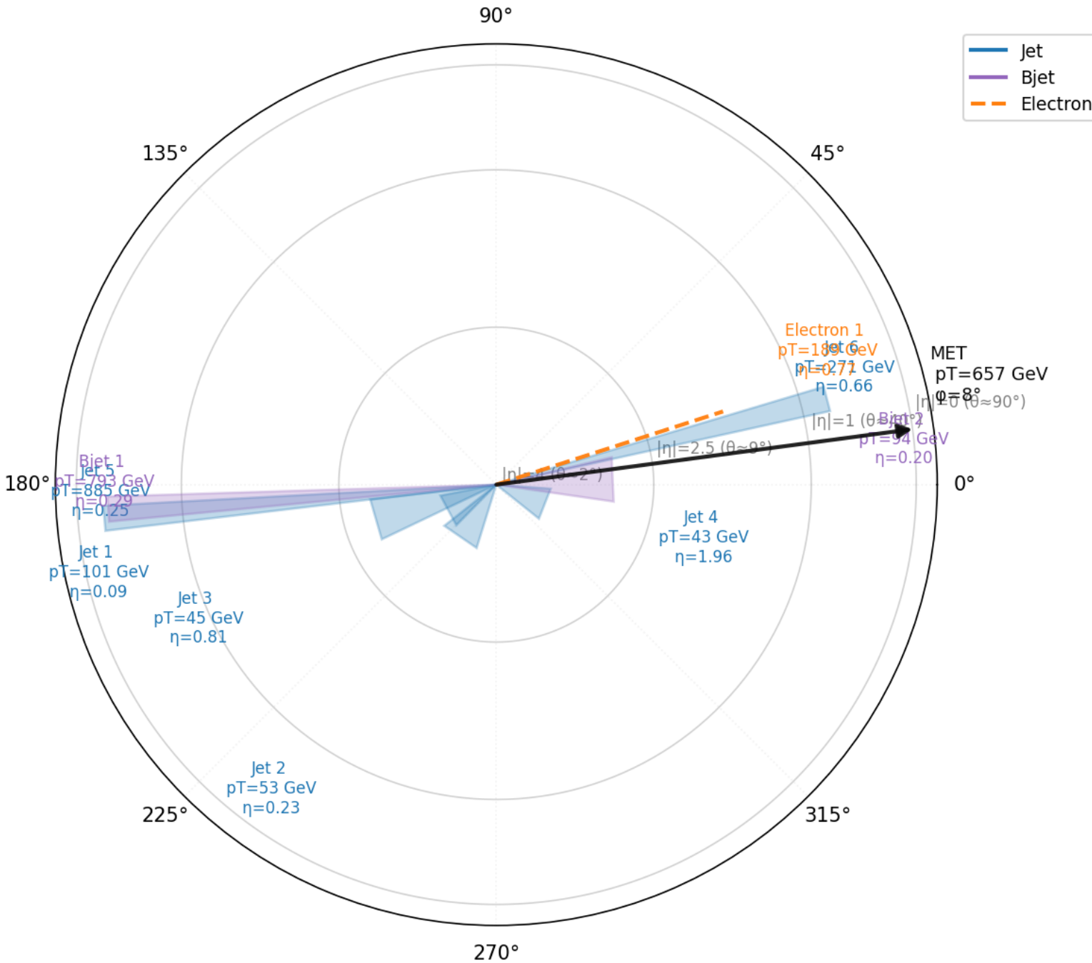
ATLAS Open Data: Z'(2 \text{ TeV}) \rightarrow t\bar{t}b\bar{b} (boosted) Event# 2736
