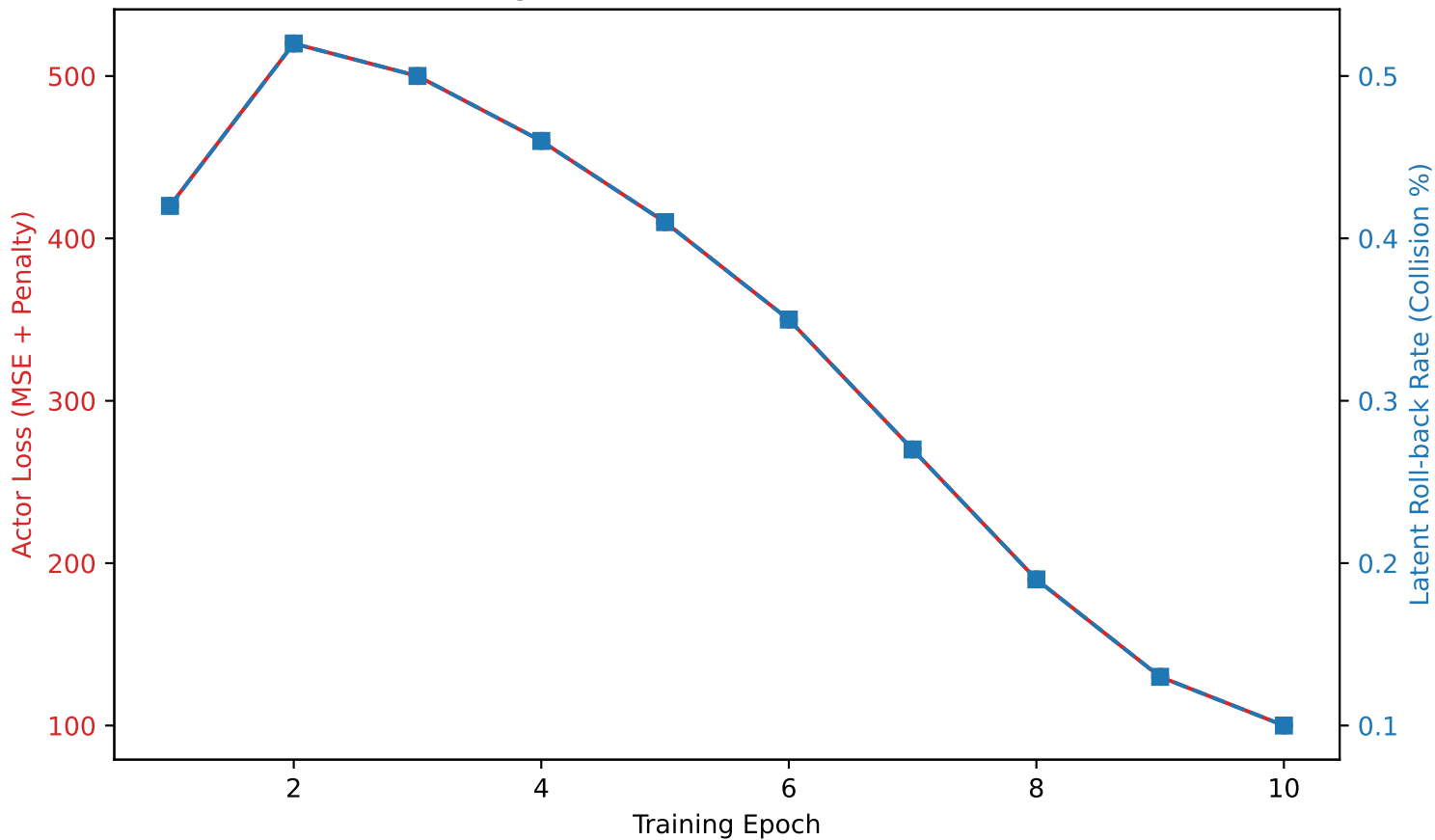
MA-WAC Training: Roll-back Rate & Actor Loss on Real Data
