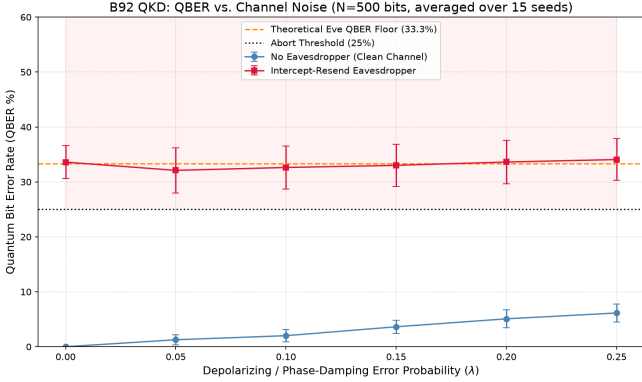
Fig. 2. Quantum Bit Error Rate (QBER) in the B92 protocol as a function of depolarizing and phase-damping noise, measured from Qiskit simulation ( N = 500 bits per noise level). The presence of an Intercept-Resend eavesdropper adds an inherent \sim 33.3\% QBER floor, demonstrating the protocol’s eavesdropping detection capability.
