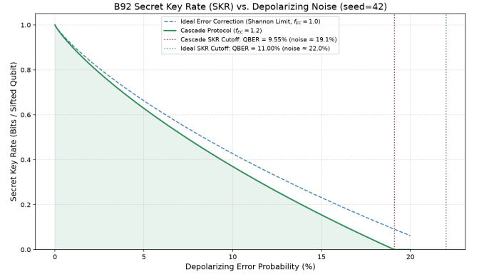
Fig. 3. Secret Key Rate (SKR) vs. Depolarizing Error Probability. The SKR rapidly falls to zero as the noise approaches the theoretical limits, demonstrating the necessity of low-noise channels for successful key distillation. The ideal curve assumes Shannon-limit error correction ( f_{EC} = 1.0 ), while the practical curve uses Cascade ( f_{EC} = 1.2 ).
