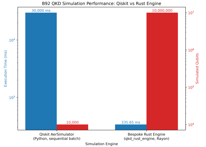
Fig. 1. Performance comparison between the sequential Qiskit Python simulation ( N = 10,000 ) and the highly-parallelized Rust Simulation Engine ( N = 10,000,000 ). The Rust engine executes 1,000\times more qubits in a fraction of the time.
