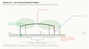
Section technical drawing
