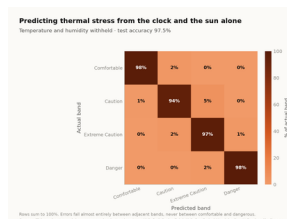
Fig07 confusion matrix
