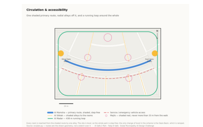
Circulation technical drawing
