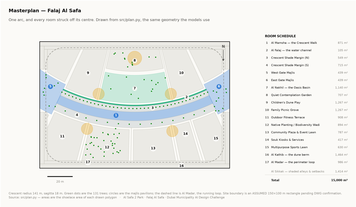
Masterplan. Technical drawing — to scale.
