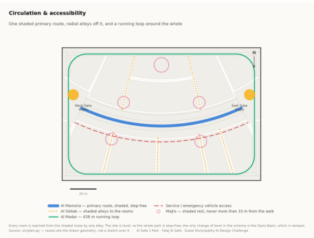
Circulation technical drawing
