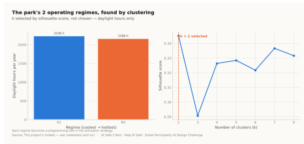
Fig08 microclimate regimes
