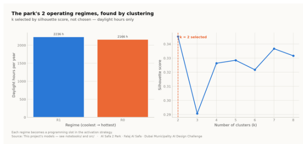
Fig08 microclimate regimes
