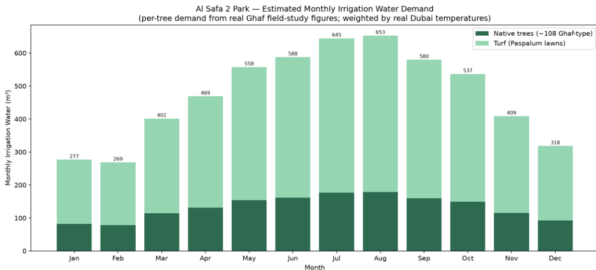
Computed monthly irrigation water demand (real Ghaf + real temperatures).
