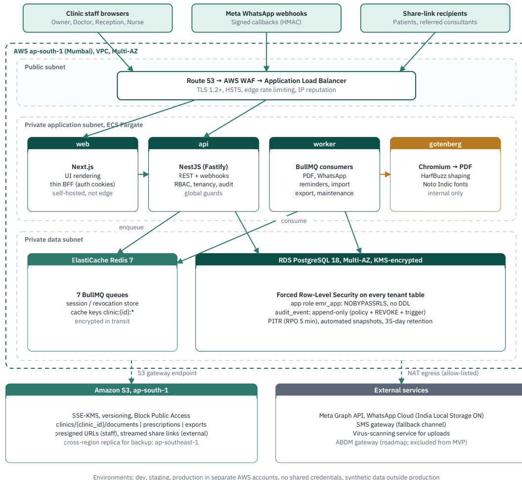
Figure 3.1, System architecture. Only the secure entry point is public. Application, database and files sit in private networks.
