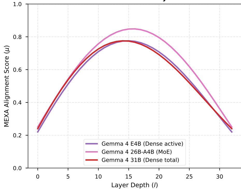
Gemma 4 Family
