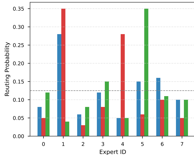
Layer 0 (Input / Lexical)
