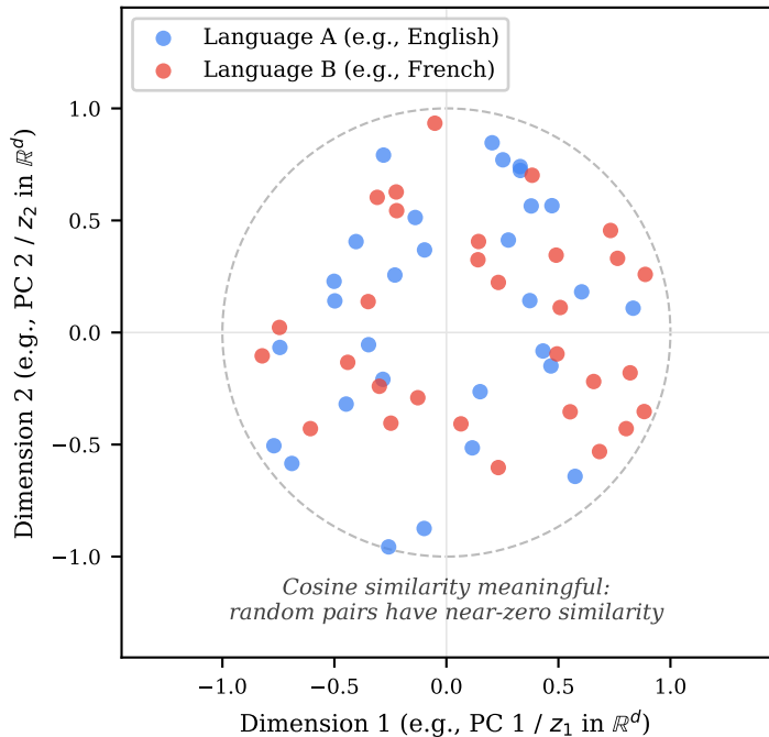
(a) Isotropic embedding space
