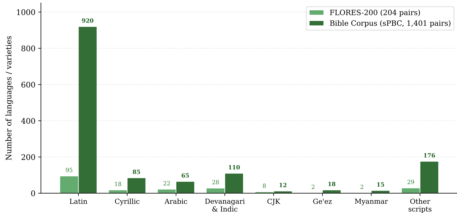
Language-script distribution across evaluation corpora
