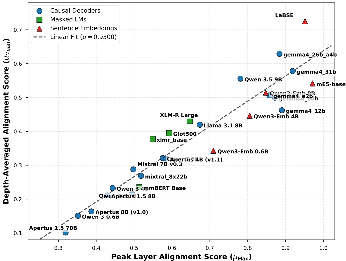
Correlation Between Peak ( \mu_{\text{Max}} ) and Mean ( \mu_{\text{Mean}} ) Alignment (All Models)
