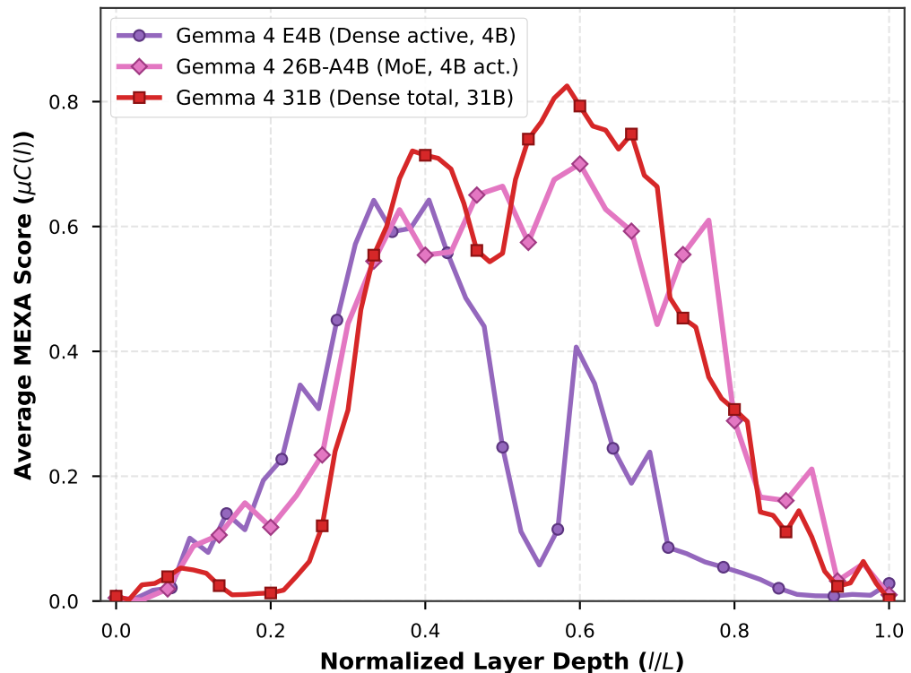
Gemma 4 Family
