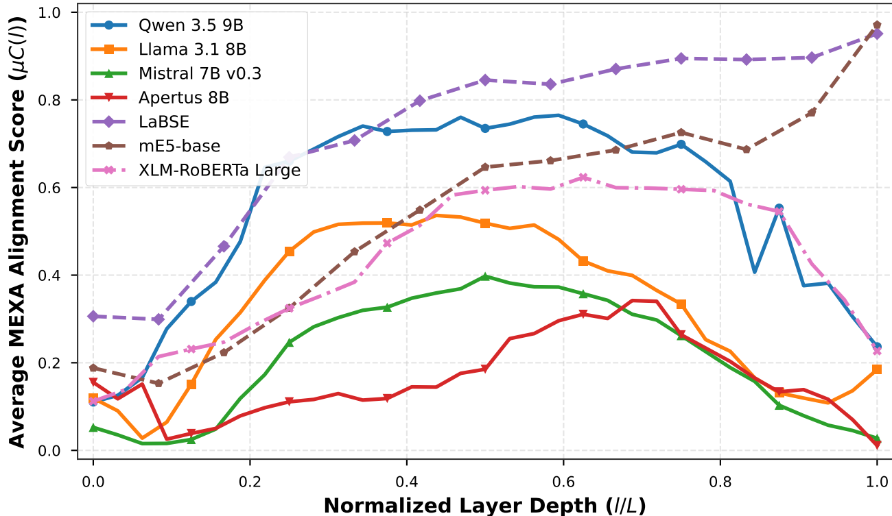
Layer-wise Cross-Lingual Alignment Trajectories (FLORES)
