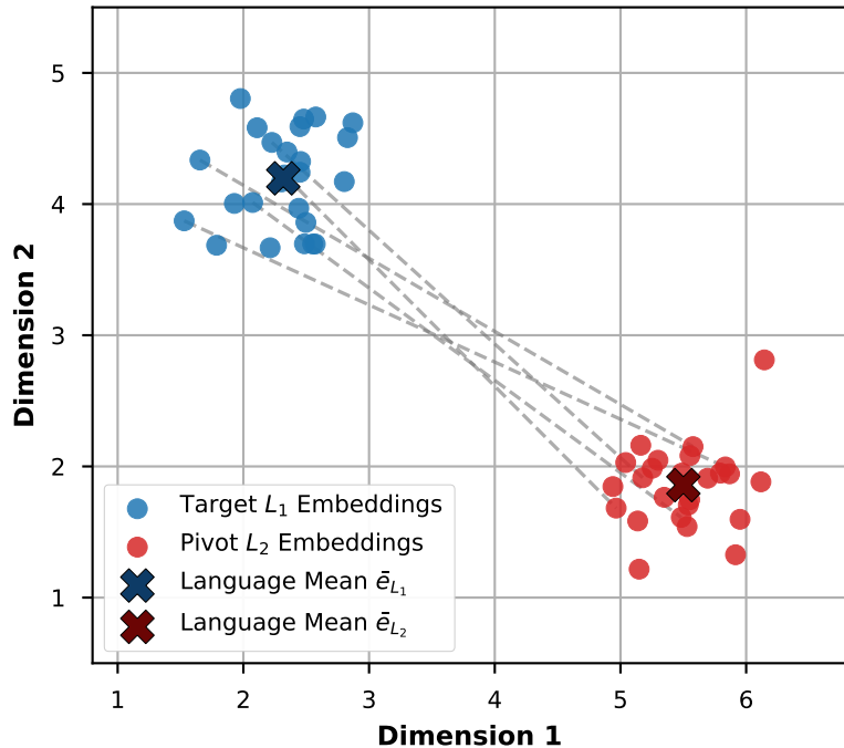
(a) Uncentered Vector Space (Dominated by Language-Identity Offsets)
