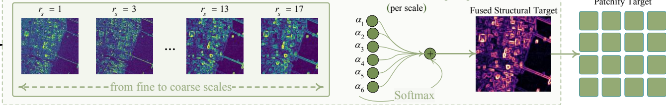
Learnable Softmax Weighting
