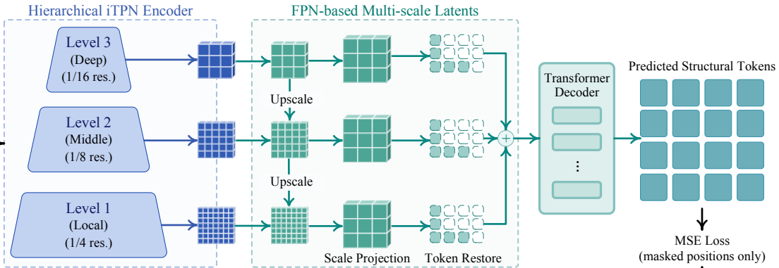
Multi-scale SAR Structural Extractors
