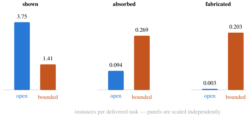
Figure 2: The result nobody designed. A bounded roster is shown roughly a third as much planted misinformation as an open directory—the filter works—and writes almost three times as much of it into the deliverable (+0.175, CI [+0.105, +0.242]). Worse, when it reaches no one it does not decline to answer: across 287 and 286 delivered tasks the open arms fabricated a value once and the bounded arms 58 times. Filtering bad claims out before they arrive removes the second source that would have caught them, so the redundancy argument of §2 shows up here as a failure mode rather than as a benefit.
