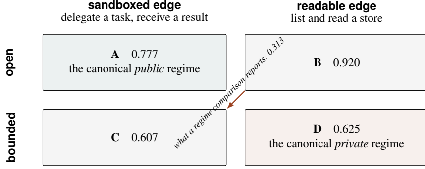
Figure 6: Requirement F_1 at the cold beat. Comparing only the diagonal confounds formation with semantics. B and C are the controls that recover both main effects: \Delta_{\text{formation}} = \frac{1}{2}[(A - C) + (B - D)] = 0.232 and \Delta_{\text{semantics}} = \frac{1}{2}[(B - A) + (D - C)] = 0.080 , summing to the 0.313 a regime comparison would report as one number. C is not a contrivance: a trusted counterpart that answers rather than exposes is the common case inside organizations.
