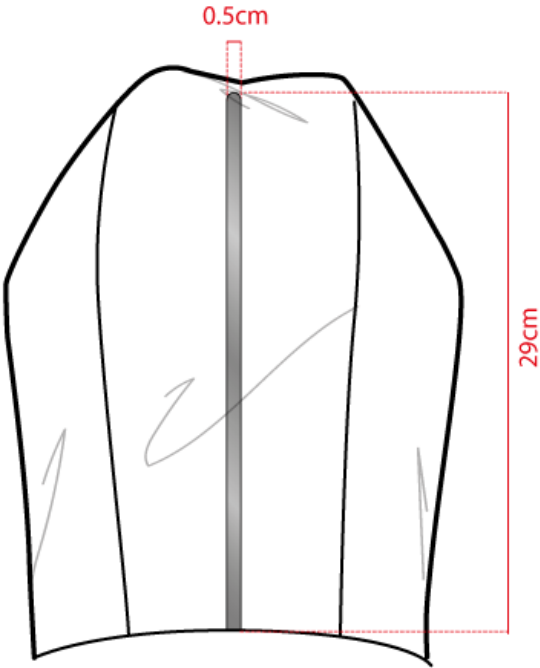
HOOD PART
