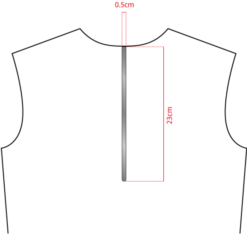
BACK PART
