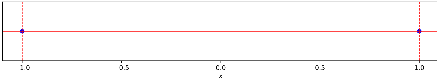
Training Points
