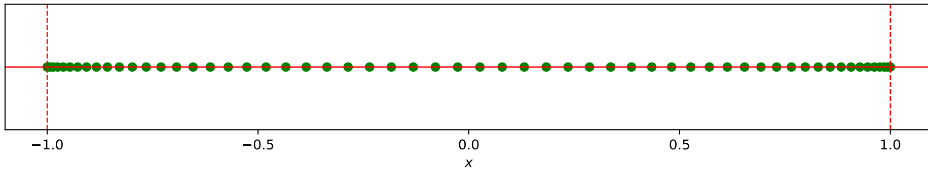
Quadrature Points
