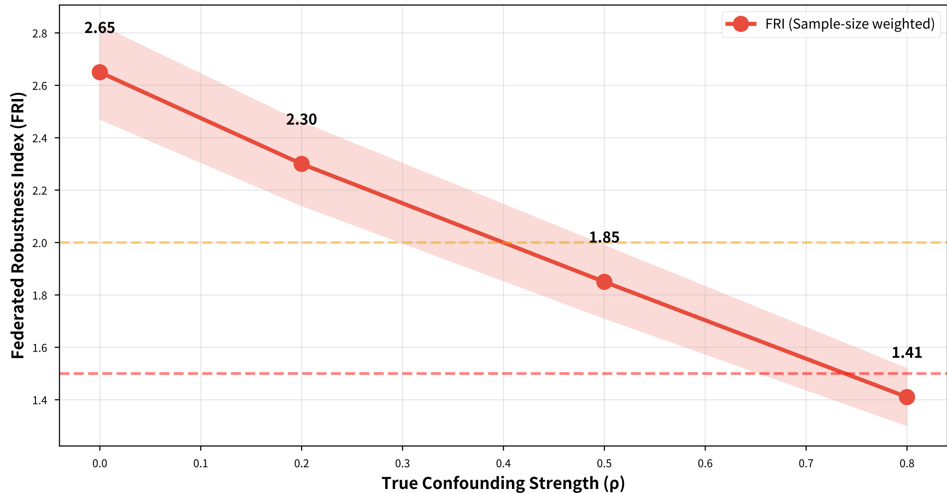
Figure 1: FRI Decreases with Confounding Strength ( r = -0.96 , p < 0.001 )
