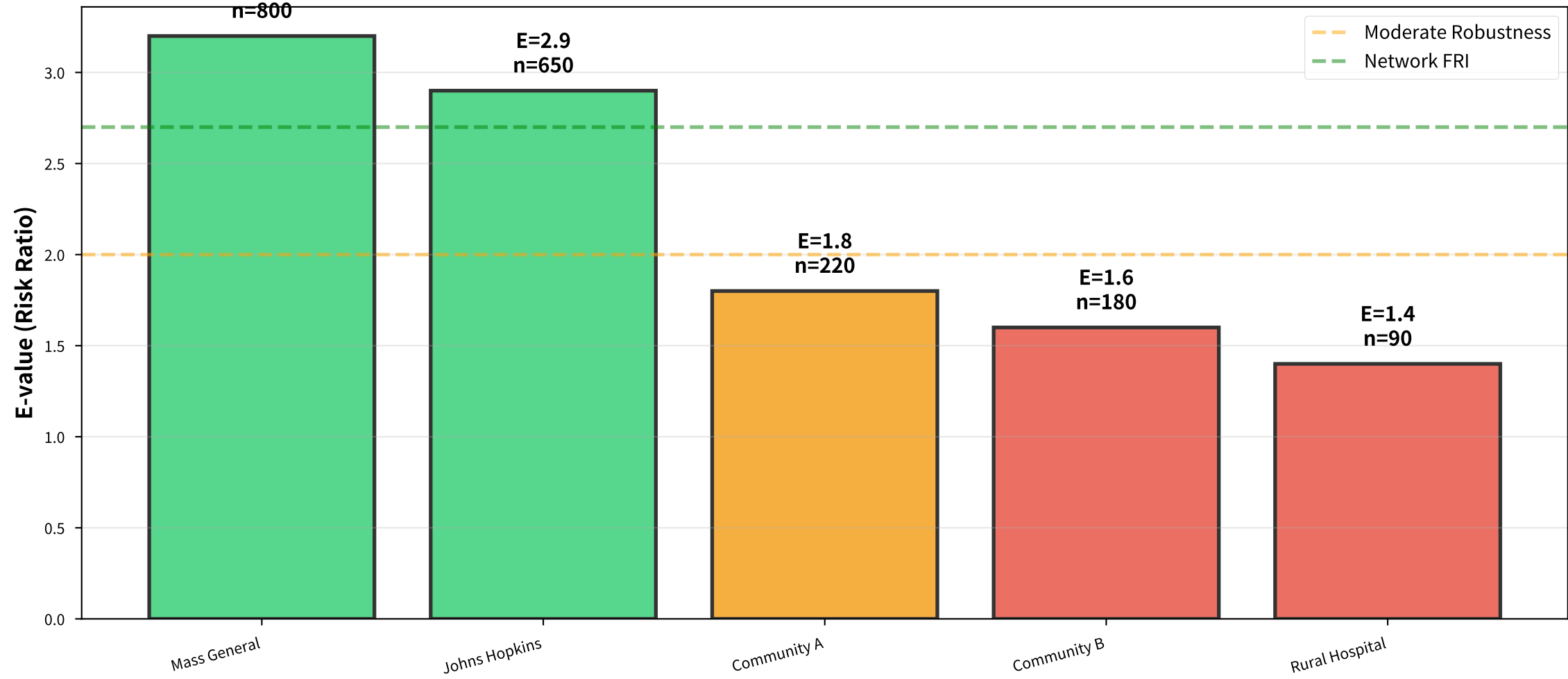
Figure 4: 5-Hospital ICU Network E-values (Vasopressor Study)
