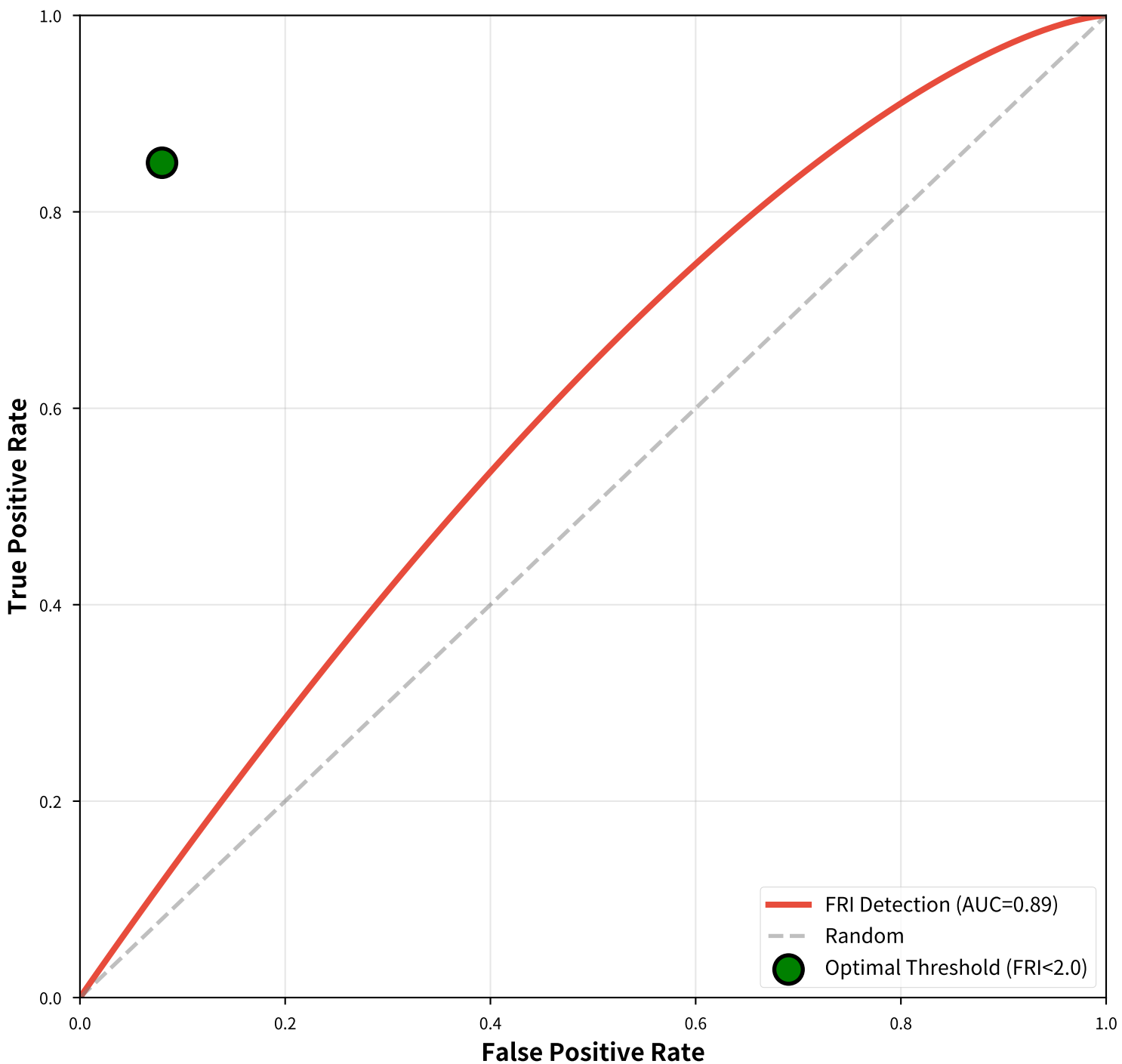
Figure 3: ROC Curve for Detecting Moderate Confounding ( \rho \geq 0.5 )
