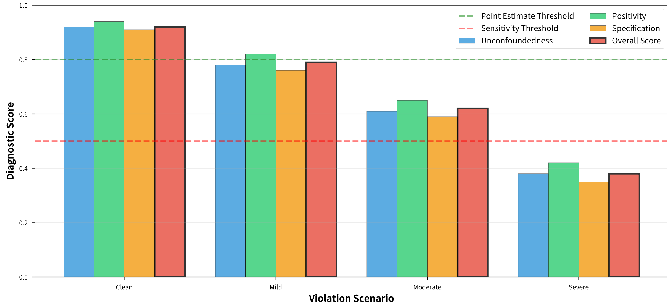
Figure 1: Diagnostic Scores Discriminate Violation Severity
