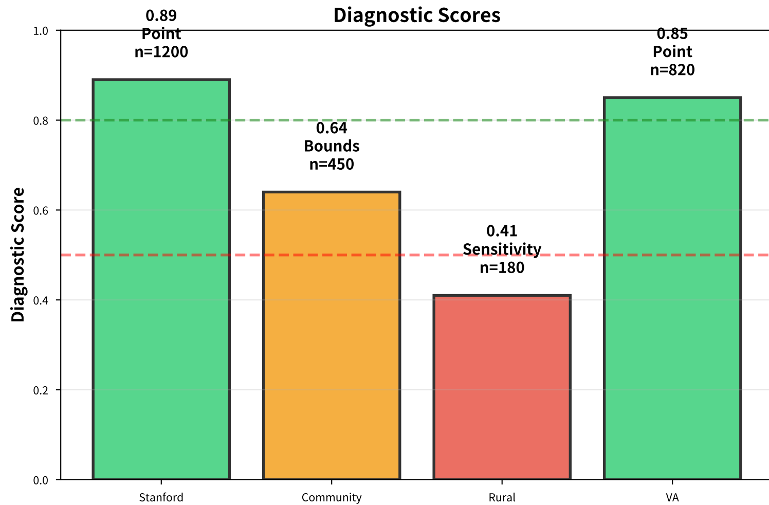
Figure 5: 4-Hospital Anticoagulation Study Heterogeneous Assumption Quality
