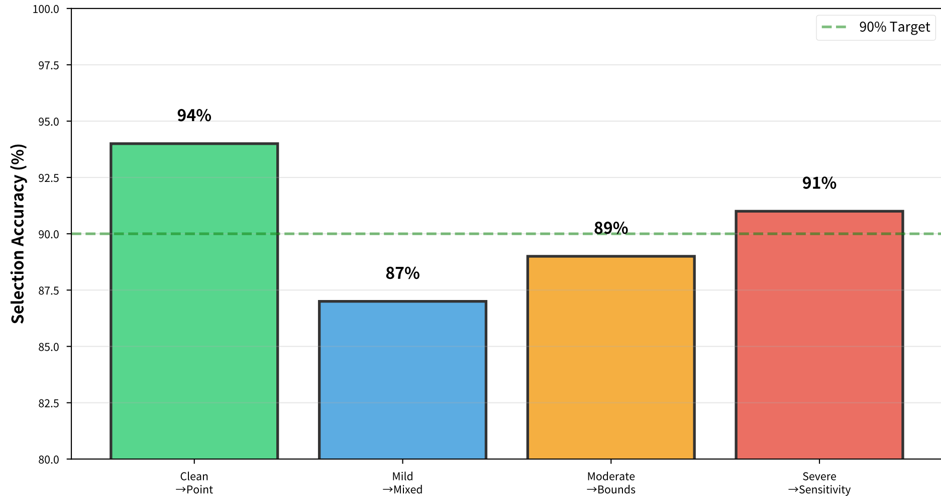
Figure 2: Automatic Mode Selection Accuracy (1,000 Iterations per Scenario)
