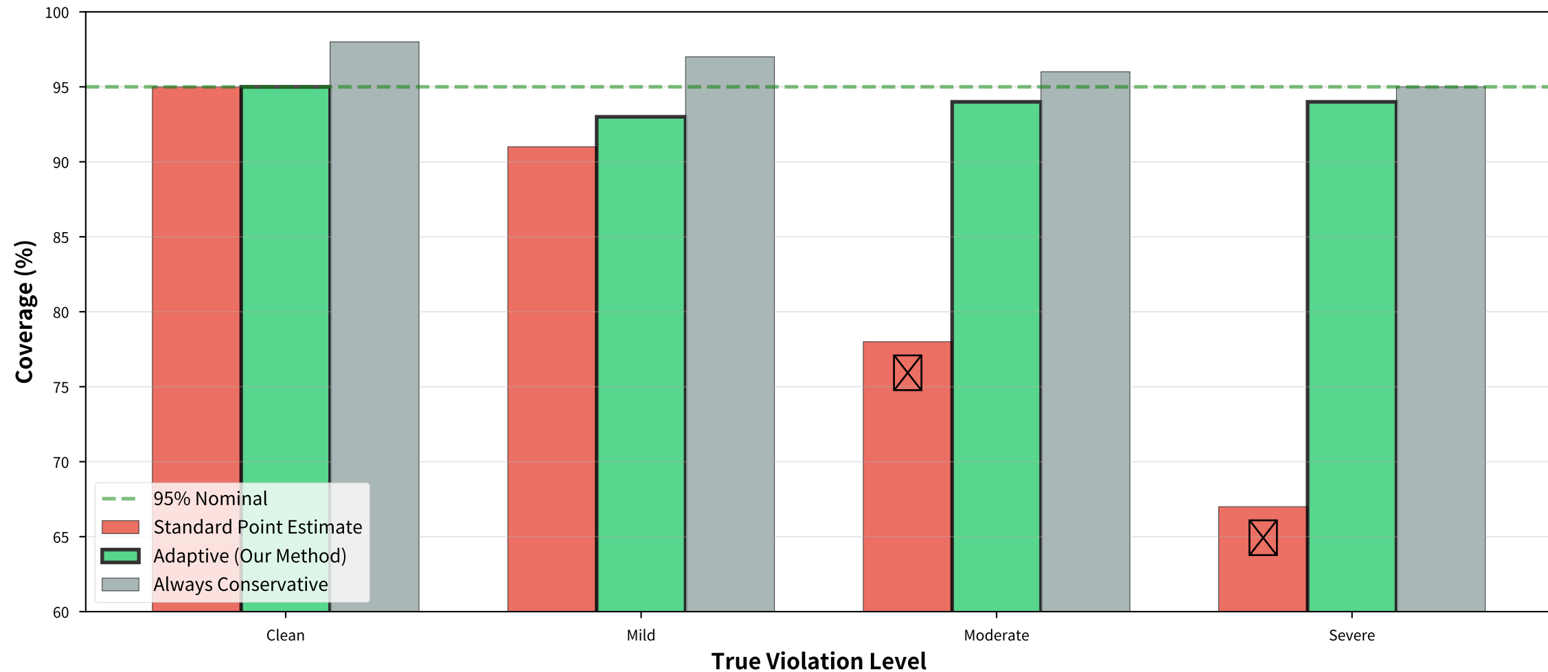
Figure 3: Coverage Maintenance Across Violation Scenarios (95% Nominal Level)
