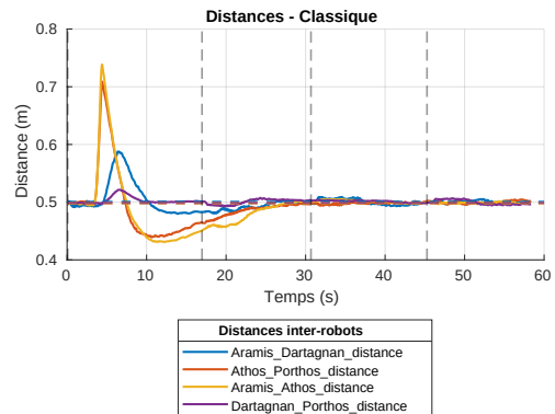
FIGURE 3 – Evolution des inter-distances
