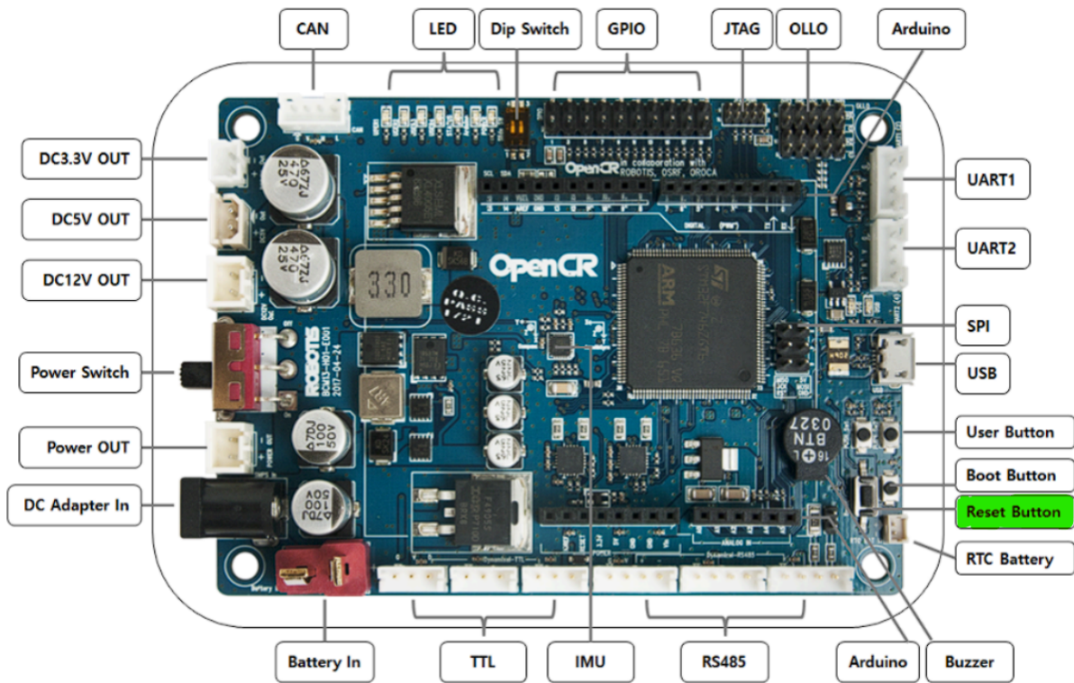
FIGURE 3.3 – Pinout OpenCR
