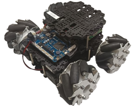
FIGURE 6.2 – TurtleBot Mecanum
