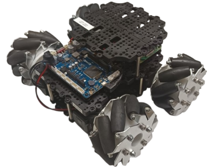
FIGURE 6.2 – TurtleBot Mecanum
