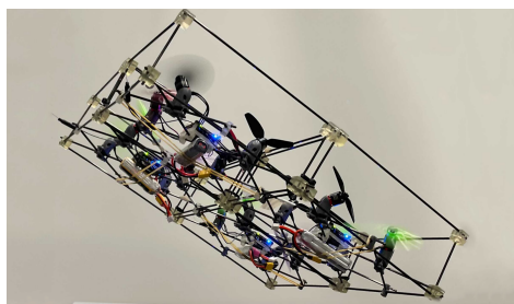
FIGURE 4.3 – ModQuad [2]
